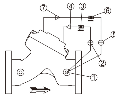
Piping Diagram
