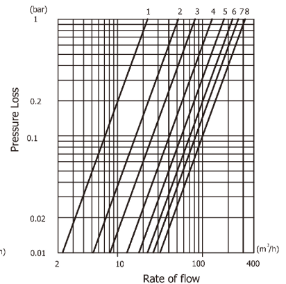
DN125mm
